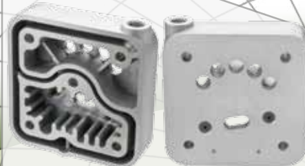
Cabeçote Inferior P/ Compressor W Mono Ø85 mm (OF 1417 / 1721) | Válvula de Lámina P/ Compressor Ø85 mm | Flap Valve Compressor Ø85 mm
